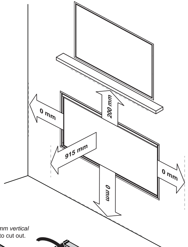
Figure 3. Clearance to Combustibles
