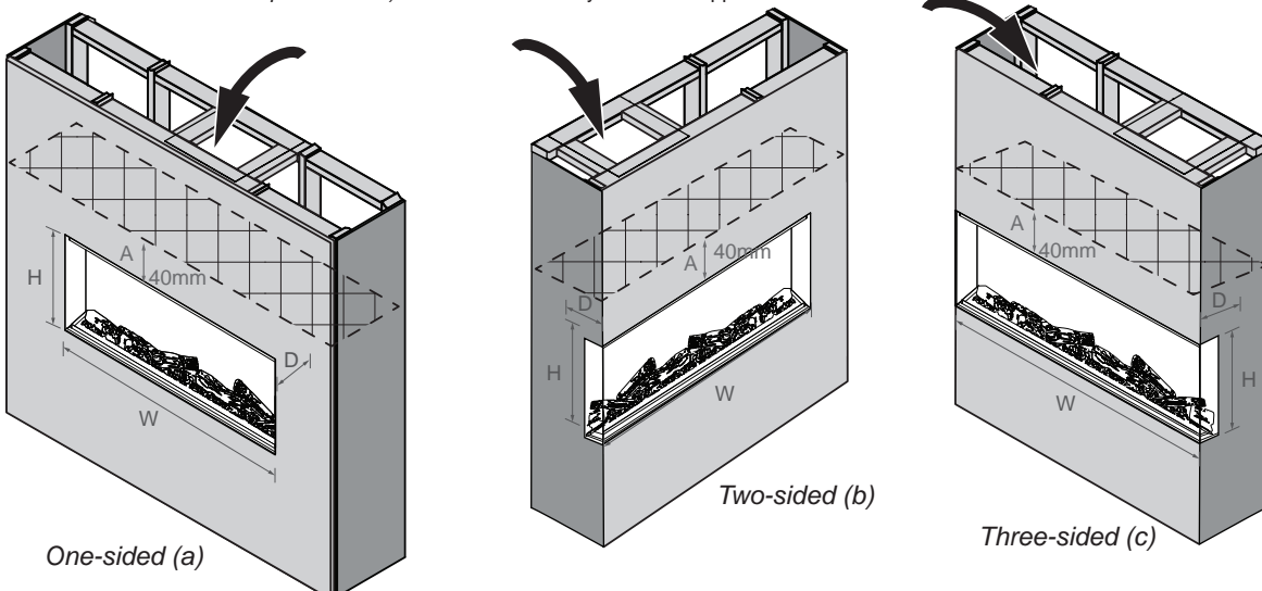
Figure 4. Cavity Dimensions
